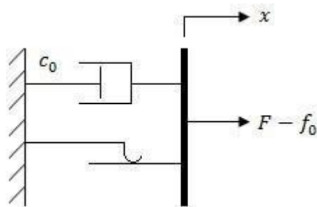
Figure 2.2 Bingham model
