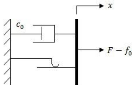
Figure 2.2 Bingham model
